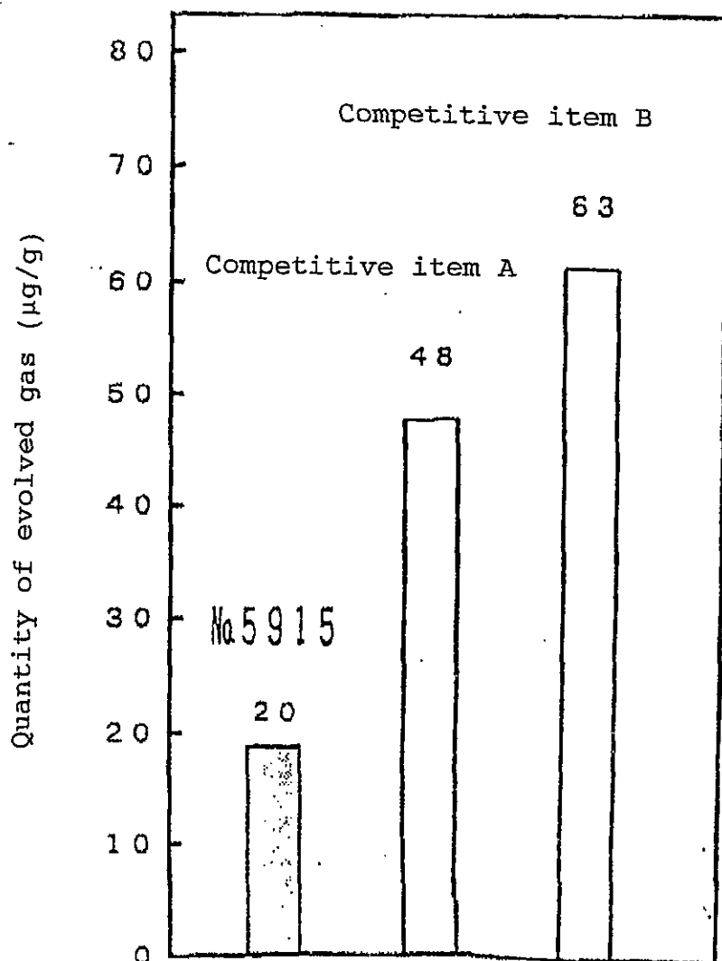
Out-gas test result
